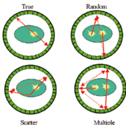
Figure 2: Illustrations of true (top, left), random (top, right), scatter (bottom, left) and multiple (bottom, right) coincidences
