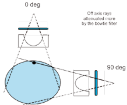
Figure 8: The effect of the bowtie filter
