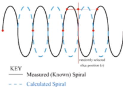
Figure 4: Diagram demonstrating interpolation
