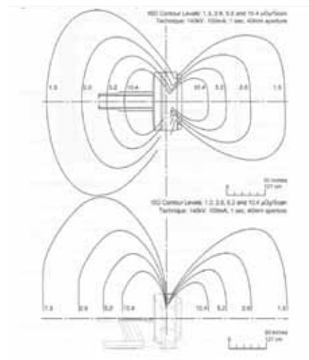
Figure 15: Typical CT 'scatter plot' depicting the path of x-rays during exposure
